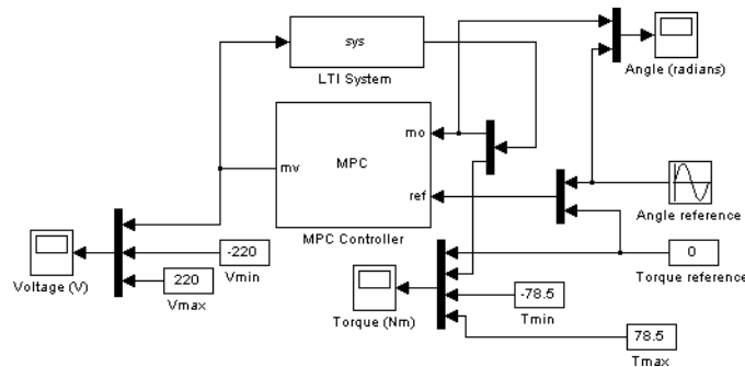
Block Diagram for the Servomechanism Example
