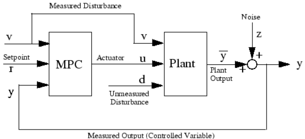
Block Diagram of a SISO Model Predictive Control Toolbox™ Application
